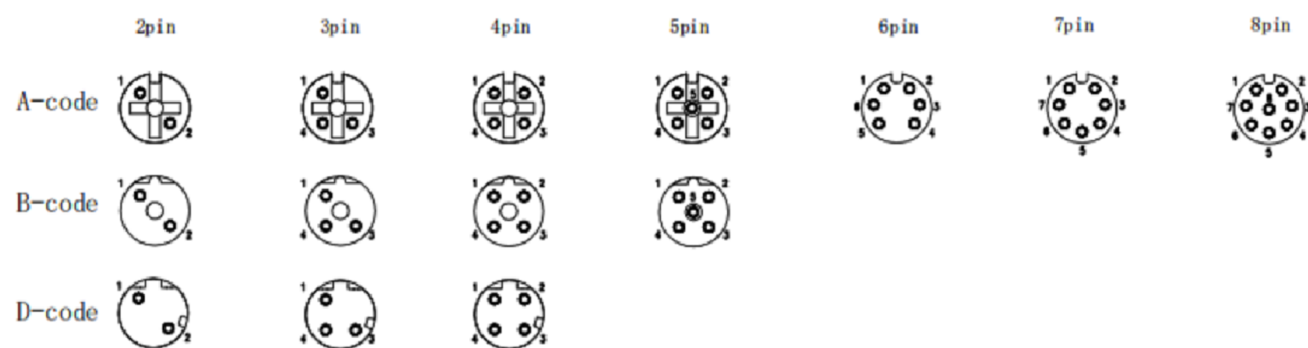
Pin assignment front view/针位分布前视图
